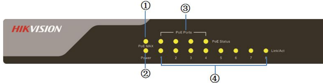
DS-3E0108P-E/M Front Panel
