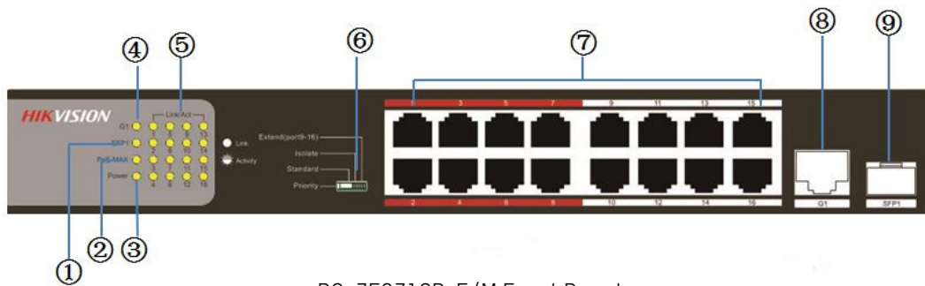
DS-3E0318P-E/M Front Panel
